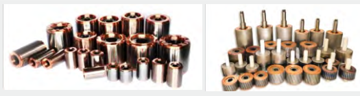
铸铜、铜焊转子电机铁芯 Cast copper, brazed rotor motor core
