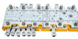
D110mm压缩机电机 三列自扣级进模 D110mm compressor motor three from the buckle progressive die
