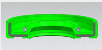
高压油封 High pressure oil seal
